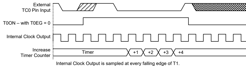
Pulse Width Measurement Mode Timing Chart (T0EG=0)
